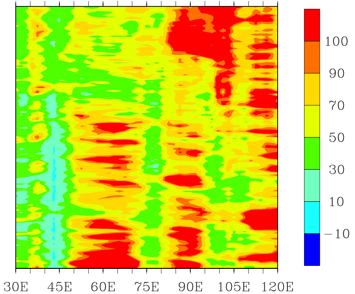
Latent Heat Net Flux(W/m 2 )
