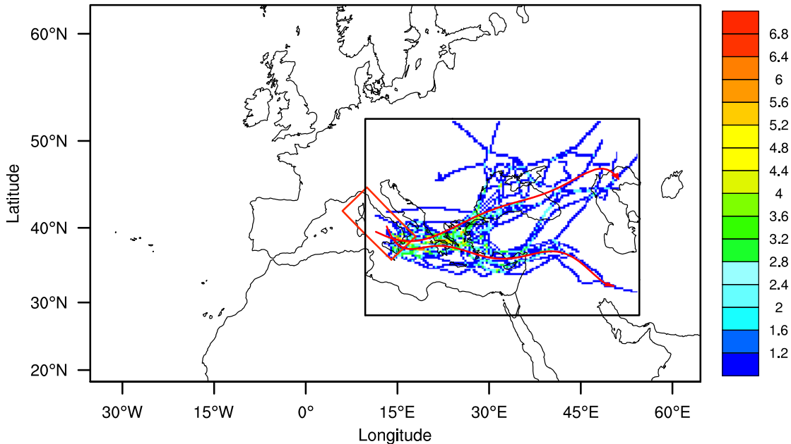
Storm Track Distribution (2d1000km) RCM20CN.RVORT.850mb.DJF (1960-1990)
