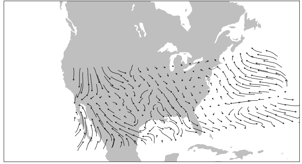
Rotated Lat-Lon - NARR
