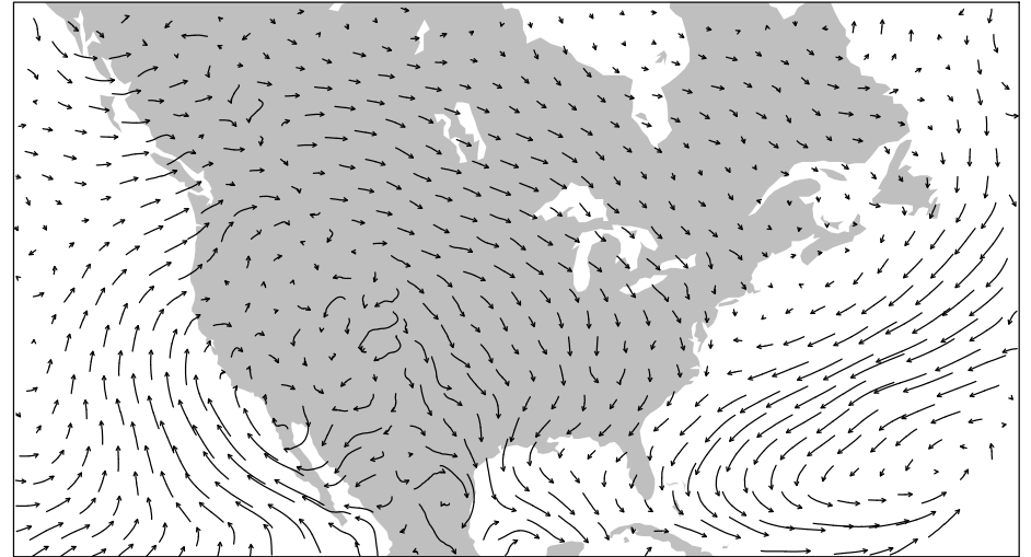
Regular Lat-Lon - NARR
