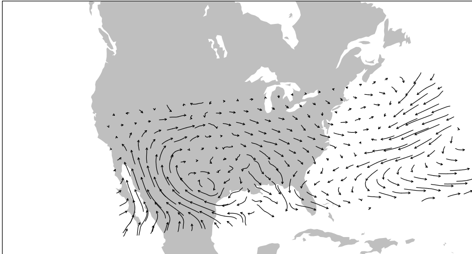
Lambert - NARR
