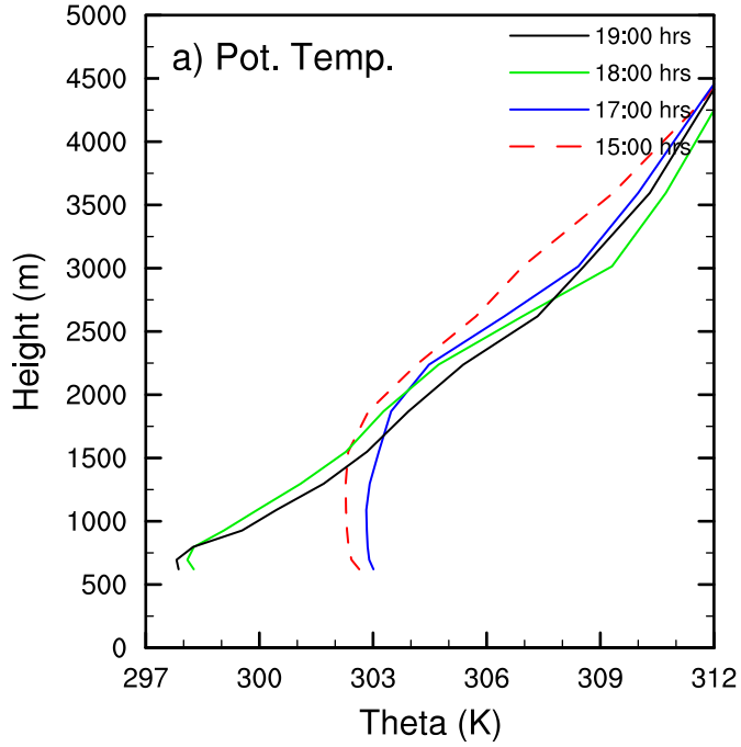
Vertical Profiles from ERA for 4 hours on 2th June 2006
